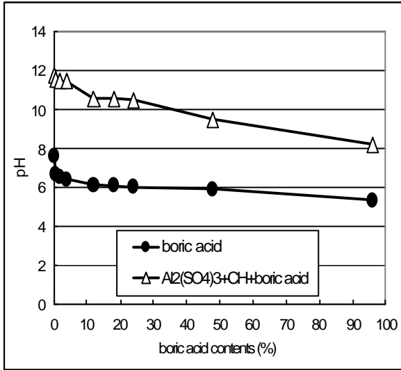
Fig.2 pH of synthetic ettringite with H 3 BO 3
