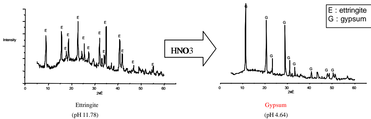
Fig.8 XRD pattern of synthetic ettringite with \text{HNO}_3
