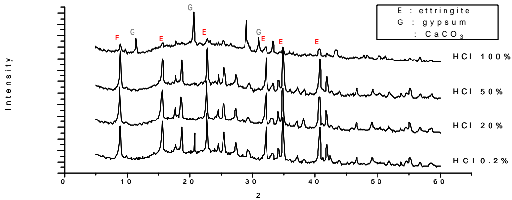
Fig.7 XRD pattern of synthetic ettringite with HCl
