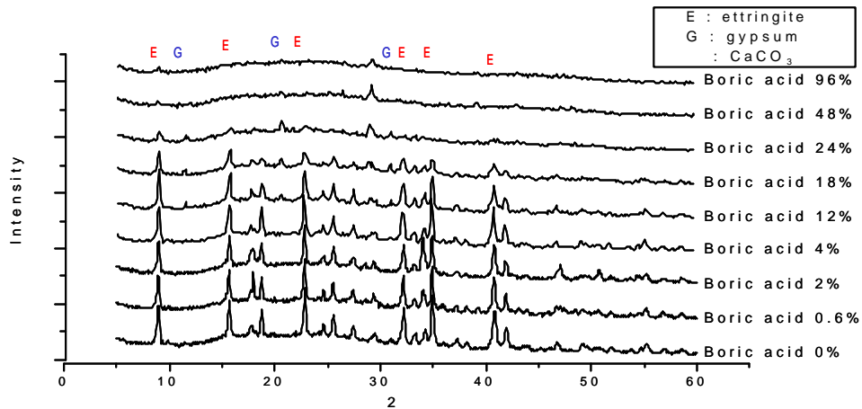
Fig.6 XRD pattern of synthetic ettringite with H_3BO_3
